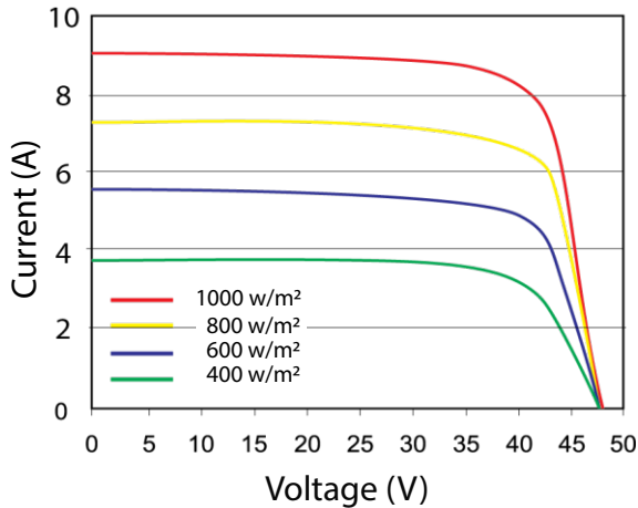
I-V curves at sun of 360-24 M at different irradiance
