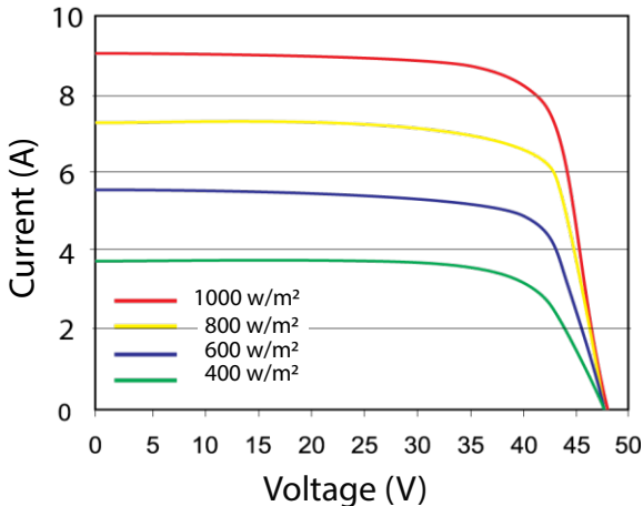
I-V curves at sun of 330-24 P at different irradiance
