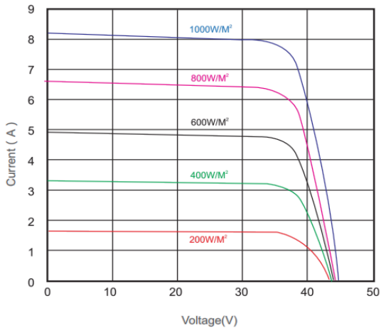
I-V curves at sun of 340-72 P at different irradiance
