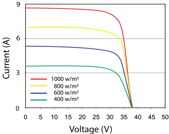
I-V curves at sun of 300-24 M DUO at different irradiance
