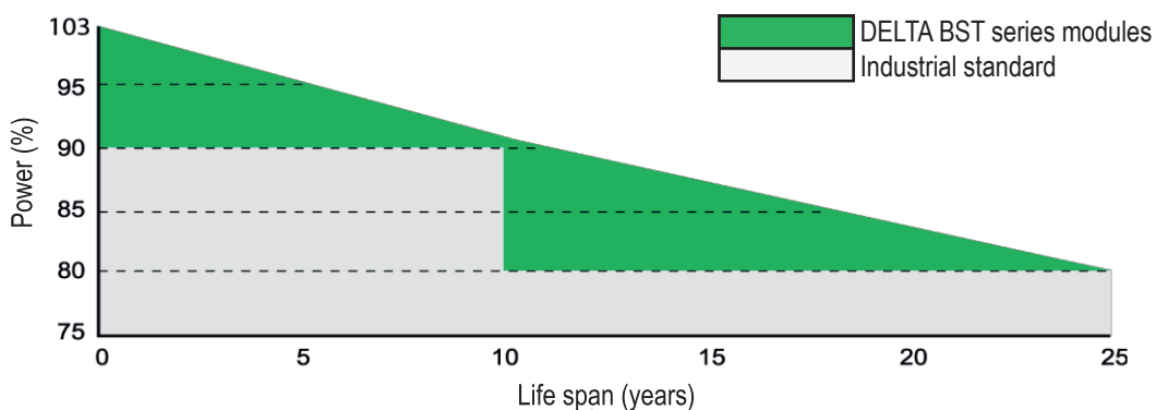
Forecasted power conservation of the solar module
