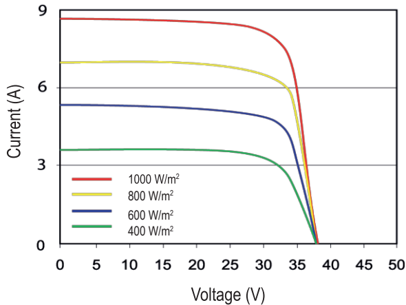
I-V curves at sun of 330-60 M at different irradiance
