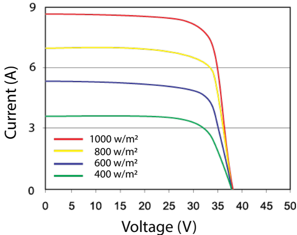
I-V curves at sun of 310-24 P at different irradiance
