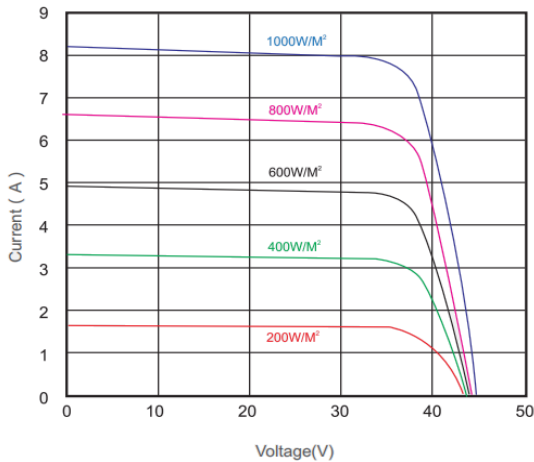
I-V curves at sun of 380-72 M at different irradiance
